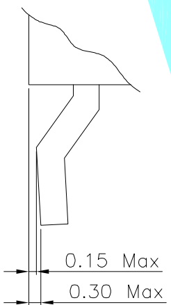
Detail of P (SCALE: 2:1)
