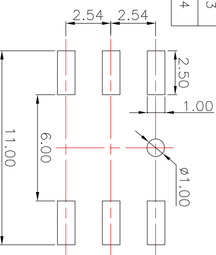
PCBLayout(Pattern Side)
